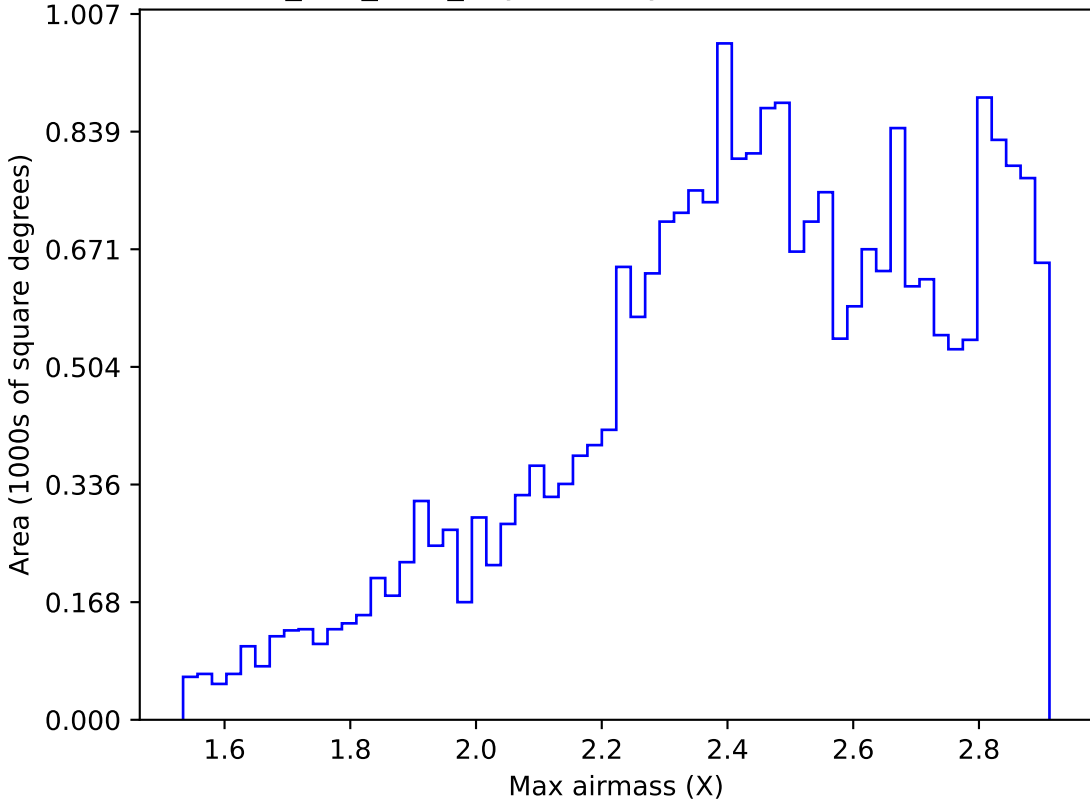
ddf_half_v3.4_10yrs All sky i band: Max airmass
