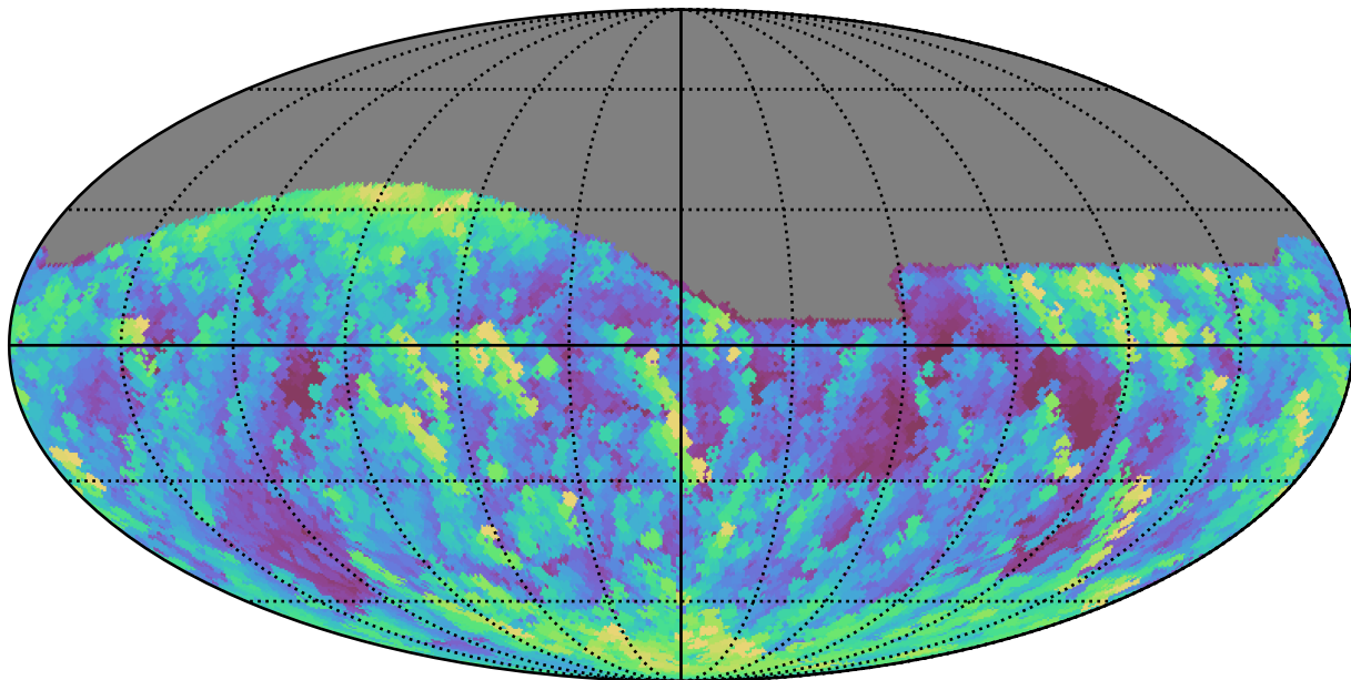
ddf_half_v3.4_10yrs All sky g band: Max airmass
