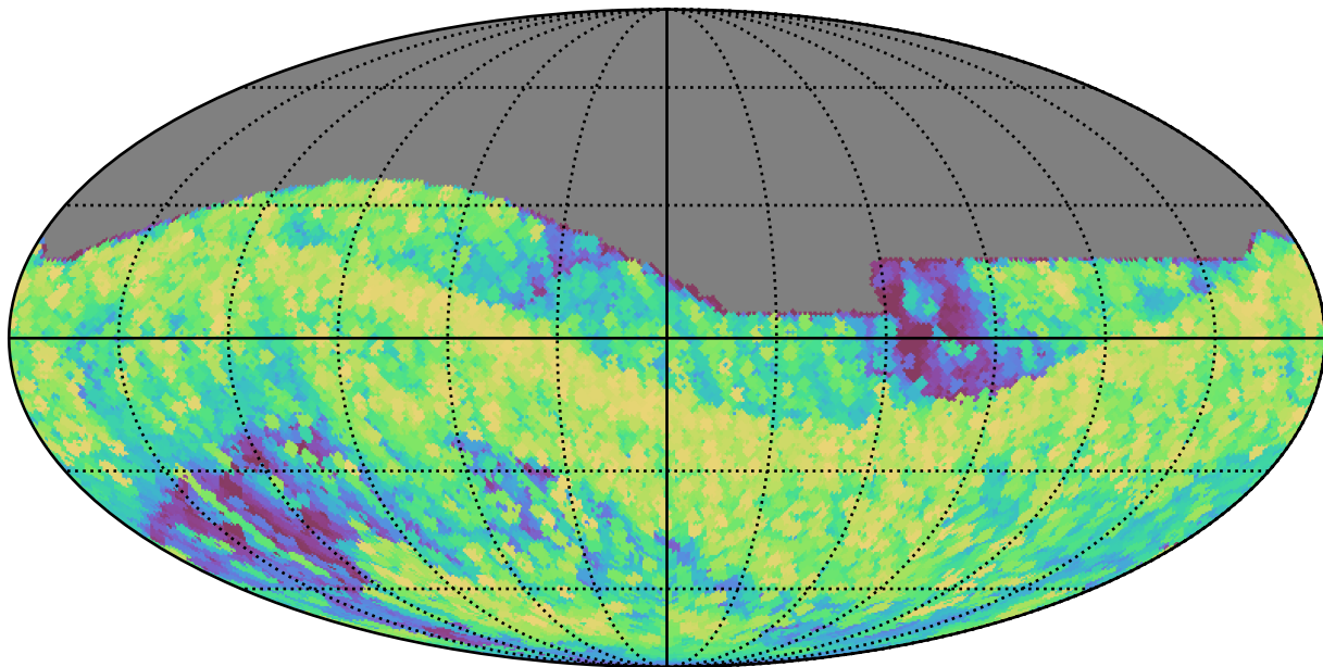
ddf_half_v3.4_10yrs All sky all bands: Max airmass
