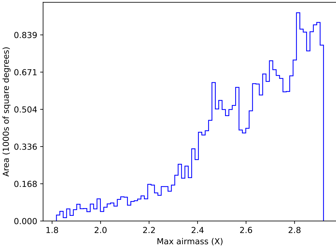
ddf_half_v3.4_10yrs All sky all bands: Max airmass
