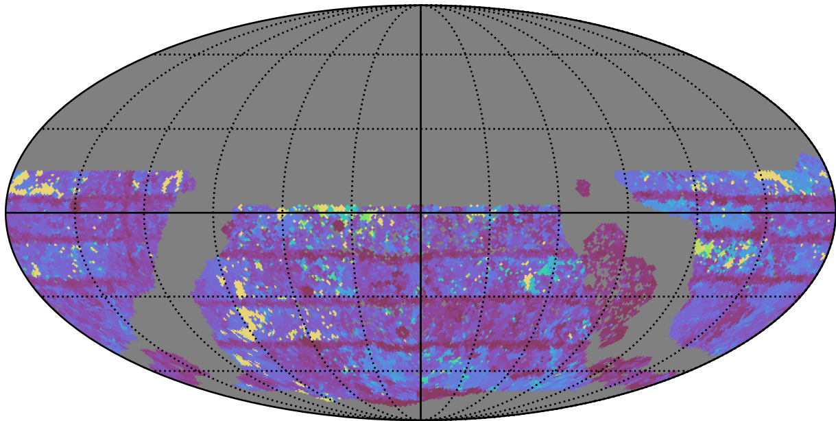
ddf_half_v3.4_10yrs WFD z band: Max Inter-Night Gap
