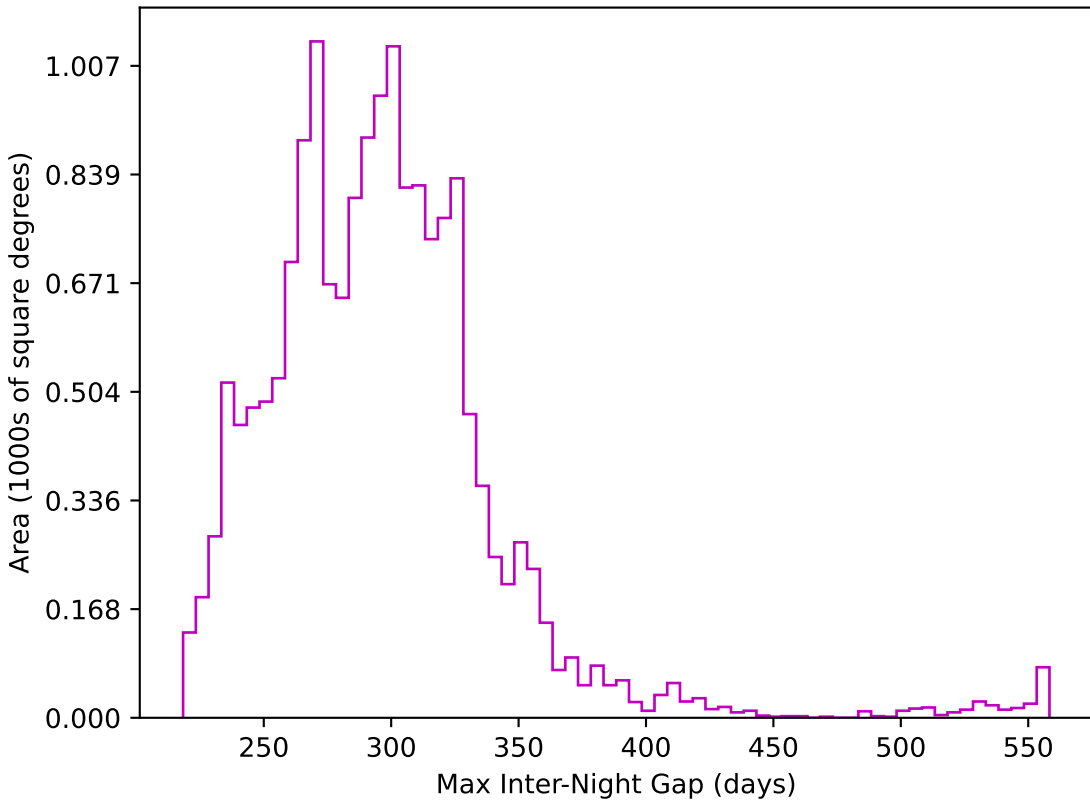
ddf_half_v3.4_10yrs WFD z band: Max Inter-Night Gap
