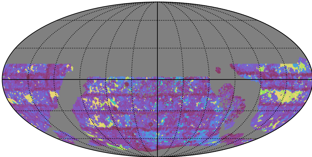
ddf_half_v3.4_10yrs WFD y band: Max Inter-Night Gap
