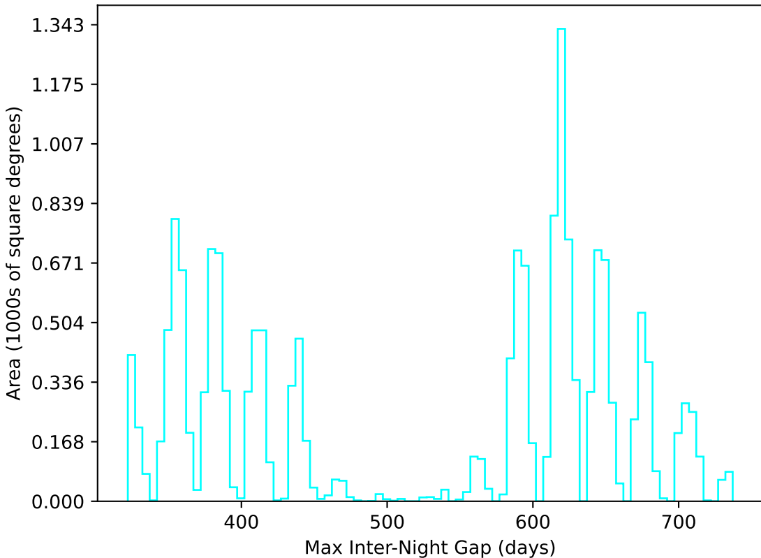
ddf_half_v3.4_10yrs WFD u band: Max Inter-Night Gap
