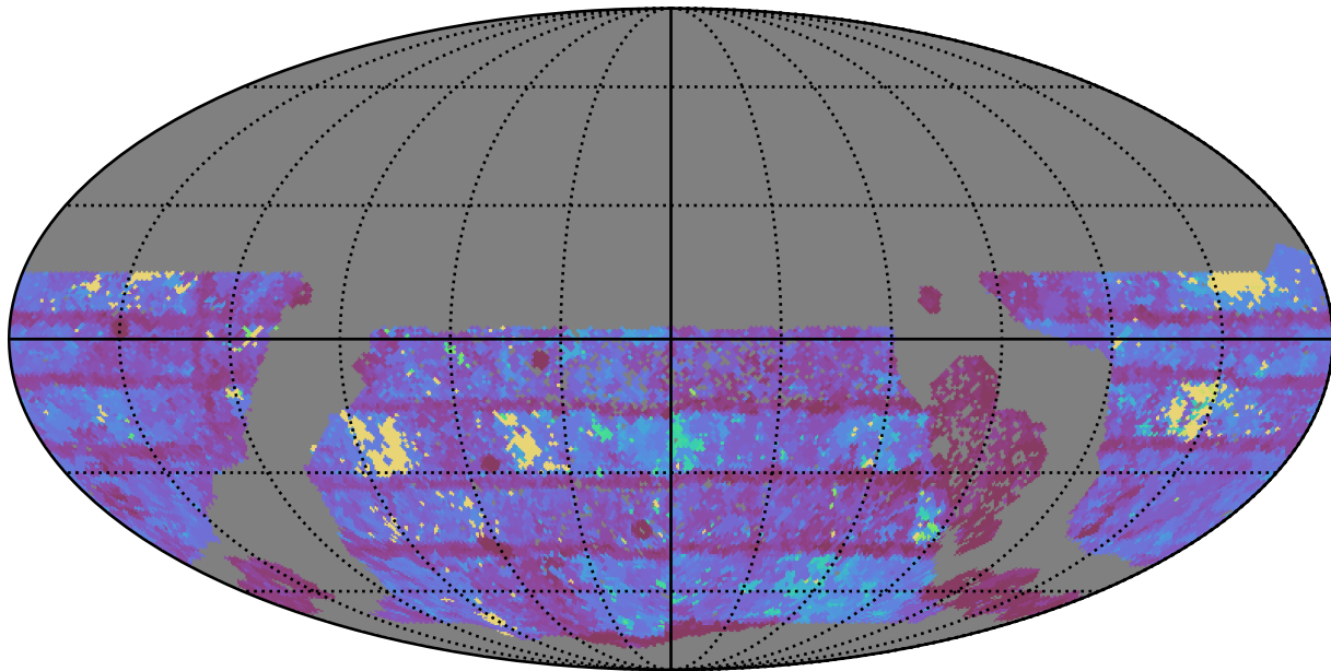
ddf_half_v3.4_10yrs WFD r band: Max Inter-Night Gap
