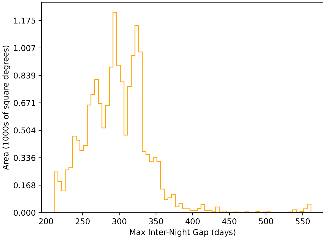
ddf_half_v3.4_10yrs WFD r band: Max Inter-Night Gap
