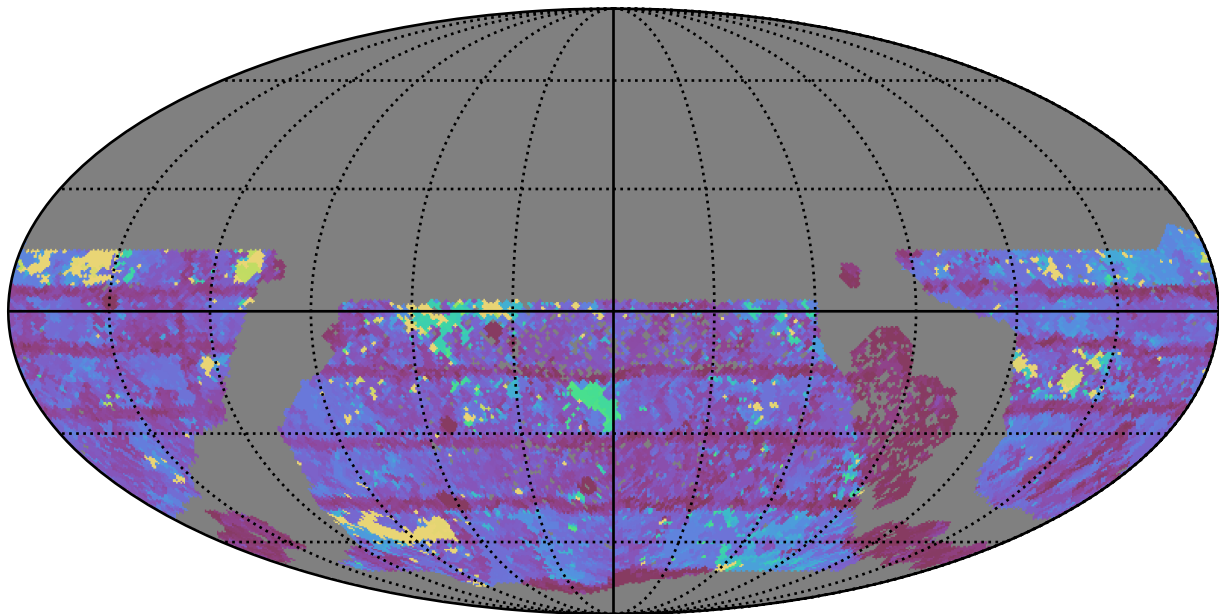
ddf_half_v3.4_10yrs WFD i band: Max Inter-Night Gap
