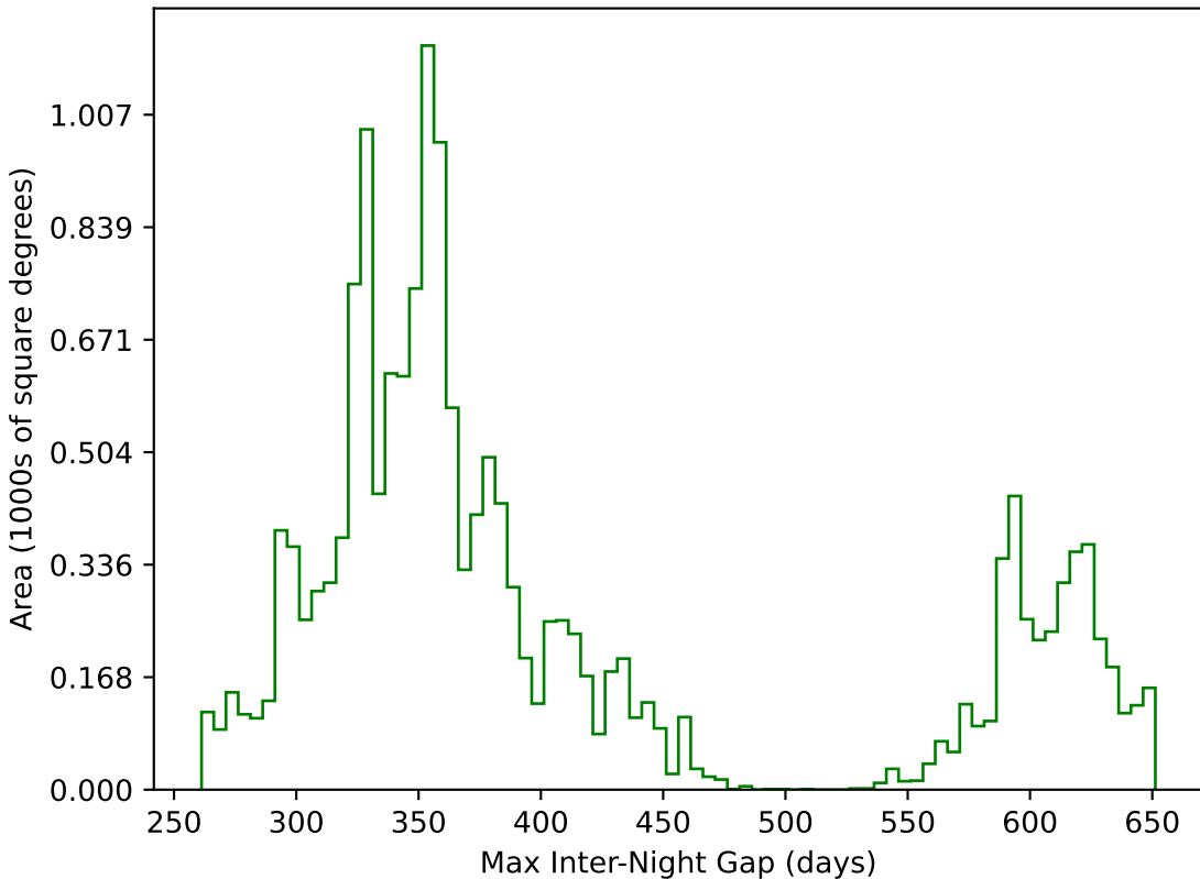
ddf_half_v3.4_10yrs WFD g band: Max Inter-Night Gap
