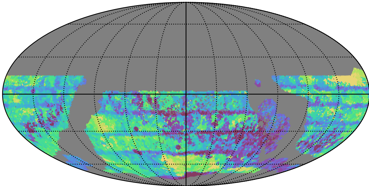
ddf_half_v3.4_10yrs WFD all bands: Max Inter-Night Gap
