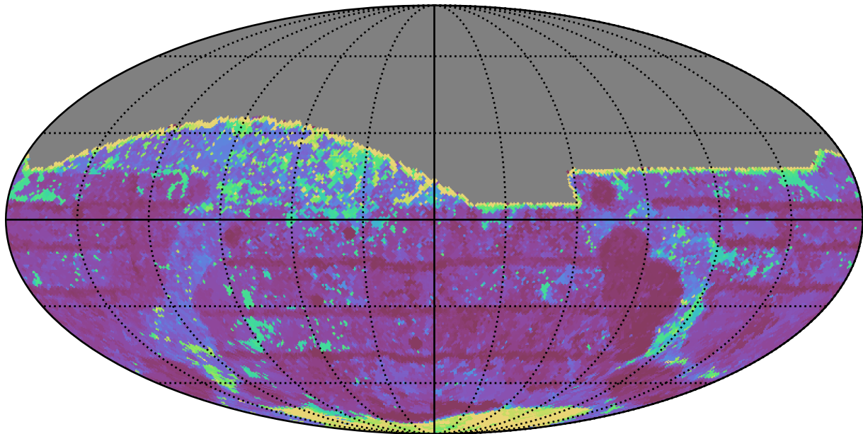
ddf_half_v3.4_10yrs All sky z band: Max Inter-Night Gap
