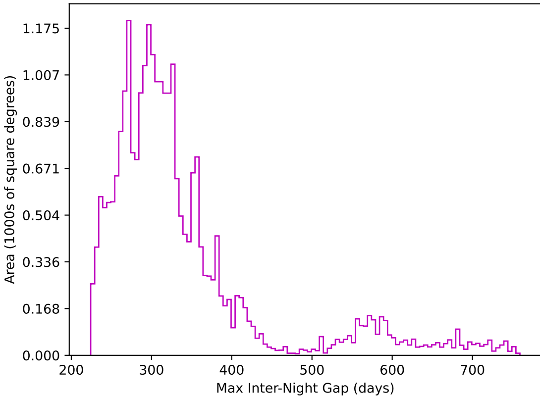
ddf_half_v3.4_10yrs All sky z band: Max Inter-Night Gap
