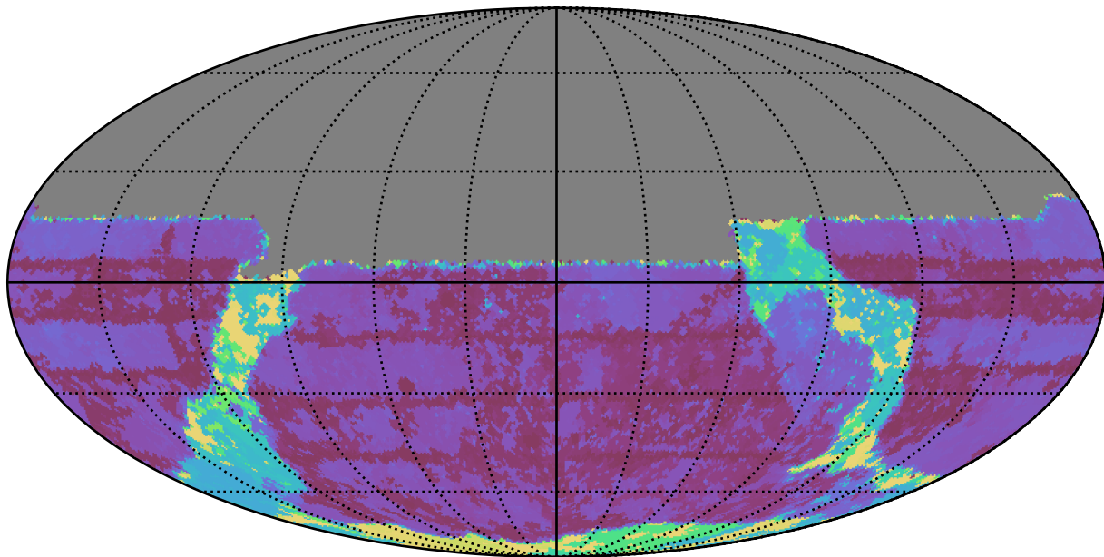
ddf_half_v3.4_10yrs All sky u band: Max Inter-Night Gap
