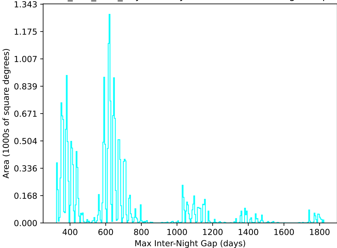
ddf_half_v3.4_10yrs All sky u band: Max Inter-Night Gap
