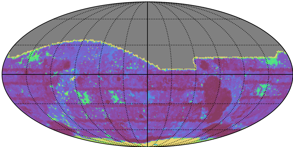
ddf_half_v3.4_10yrs All sky r band: Max Inter-Night Gap
