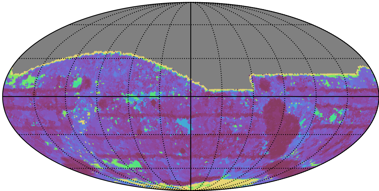
ddf_half_v3.4_10yrs All sky i band: Max Inter-Night Gap
