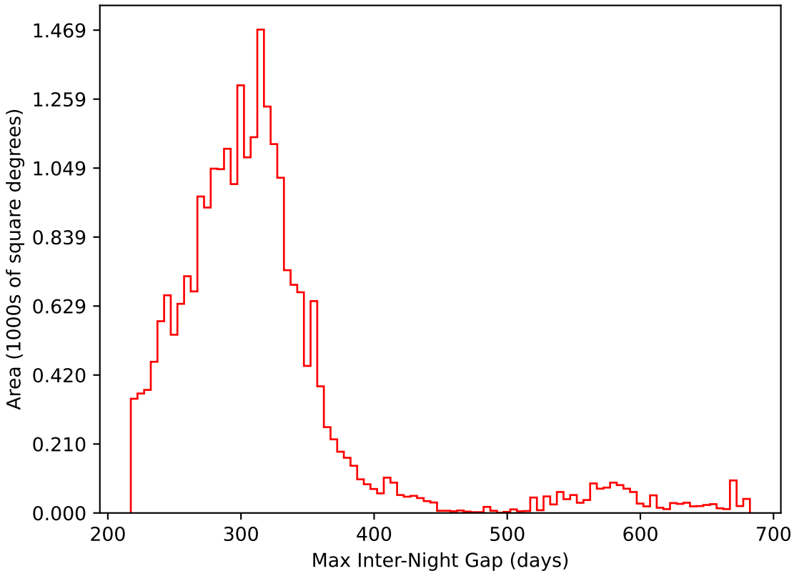
ddf_half_v3.4_10yrs All sky i band: Max Inter-Night Gap
