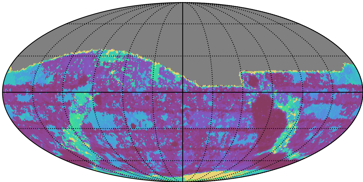
ddf_half_v3.4_10yrs All sky g band: Max Inter-Night Gap
