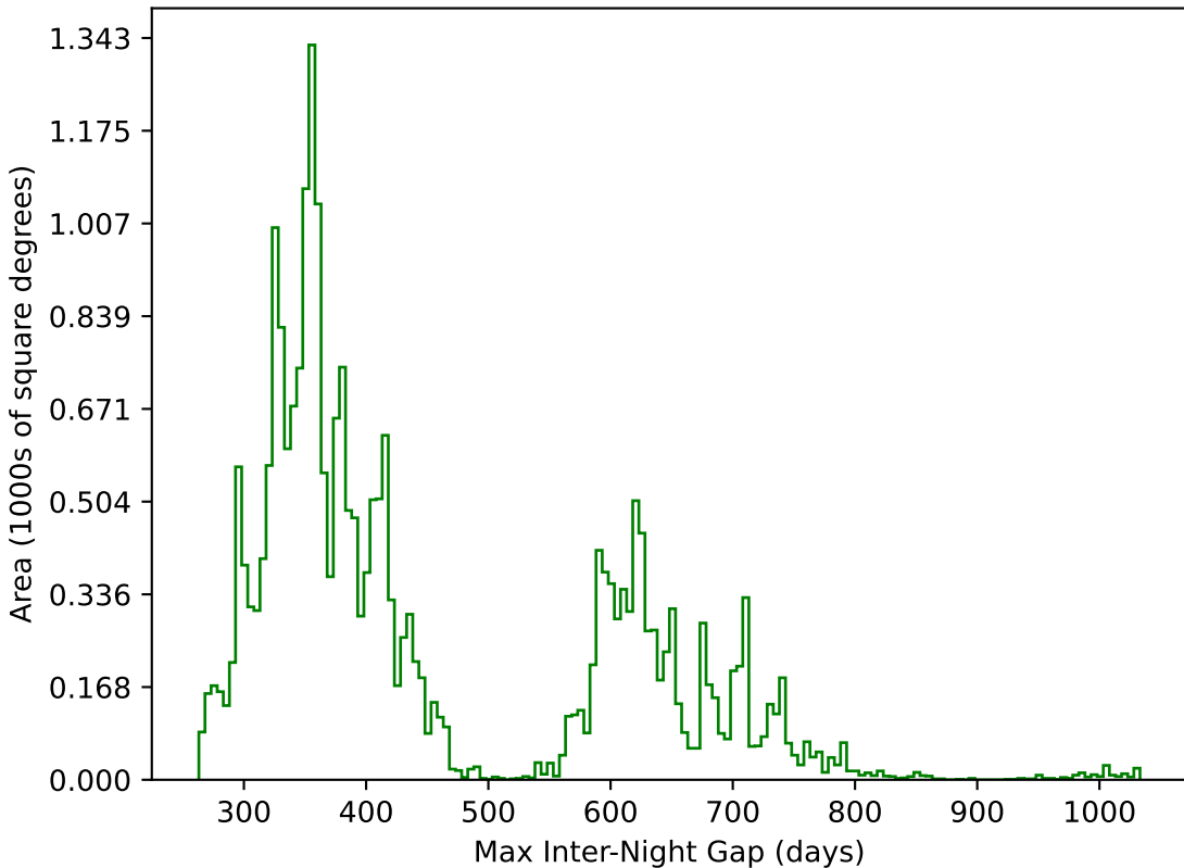
ddf_half_v3.4_10yrs All sky g band: Max Inter-Night Gap
