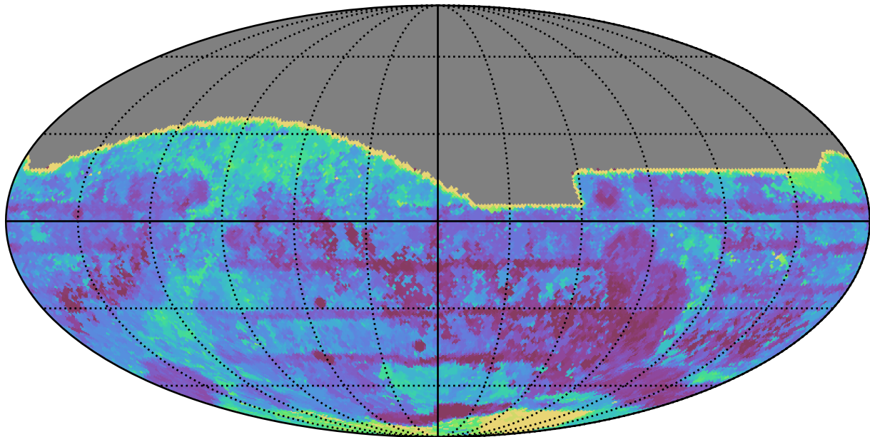
ddf_half_v3.4_10yrs All sky all bands: Max Inter-Night Gap
