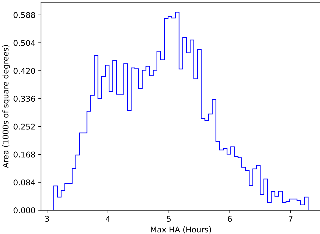
ddf_half_v3.4_10yrs WFD z band: Max HA
