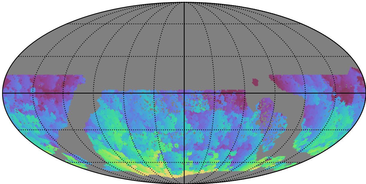
ddf_half_v3.4_10yrs WFD u band: Max HA
