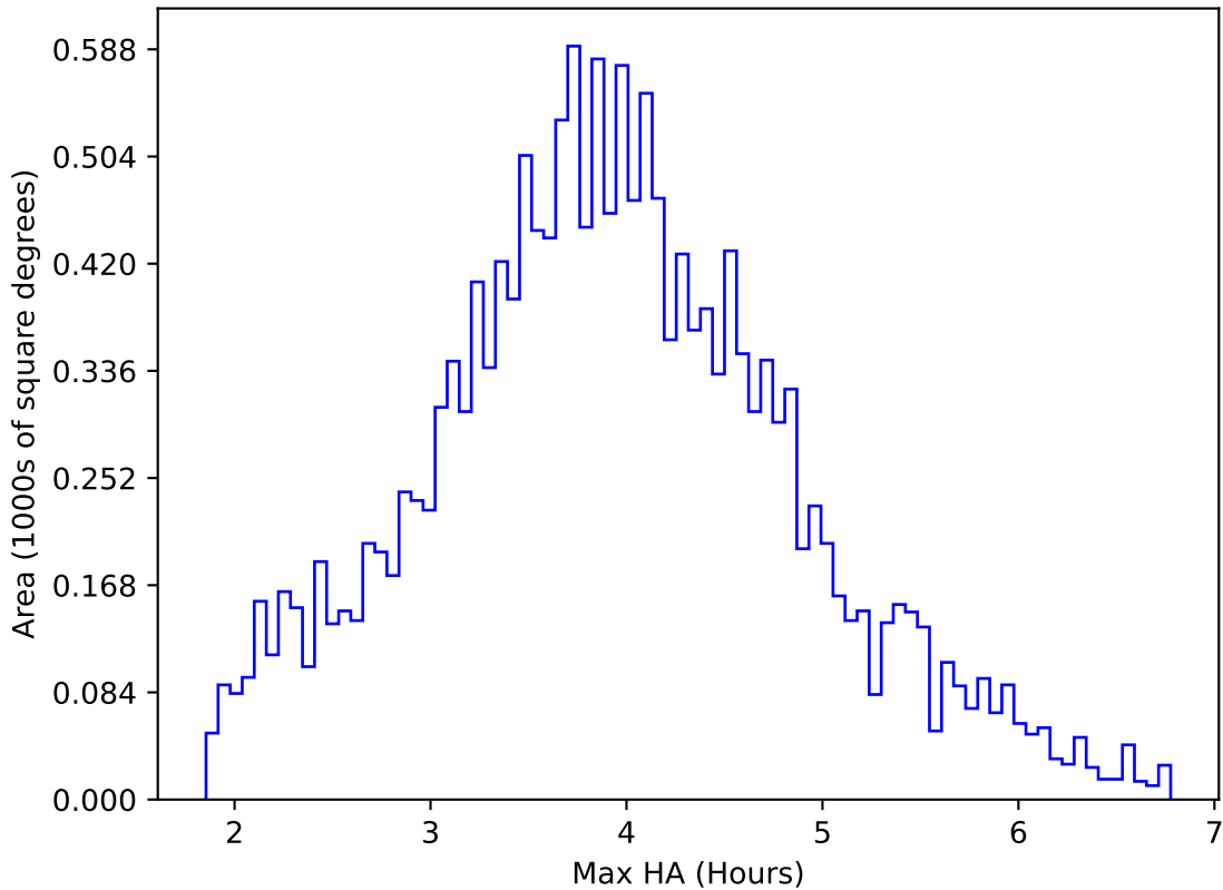
ddf_half_v3.4_10yrs WFD u band: Max HA
