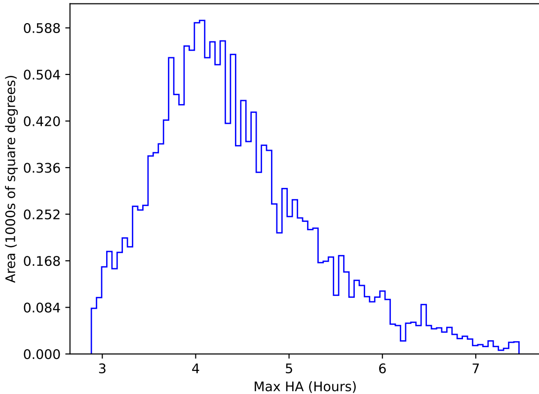
ddf_half_v3.4_10yrs WFD r band: Max HA
