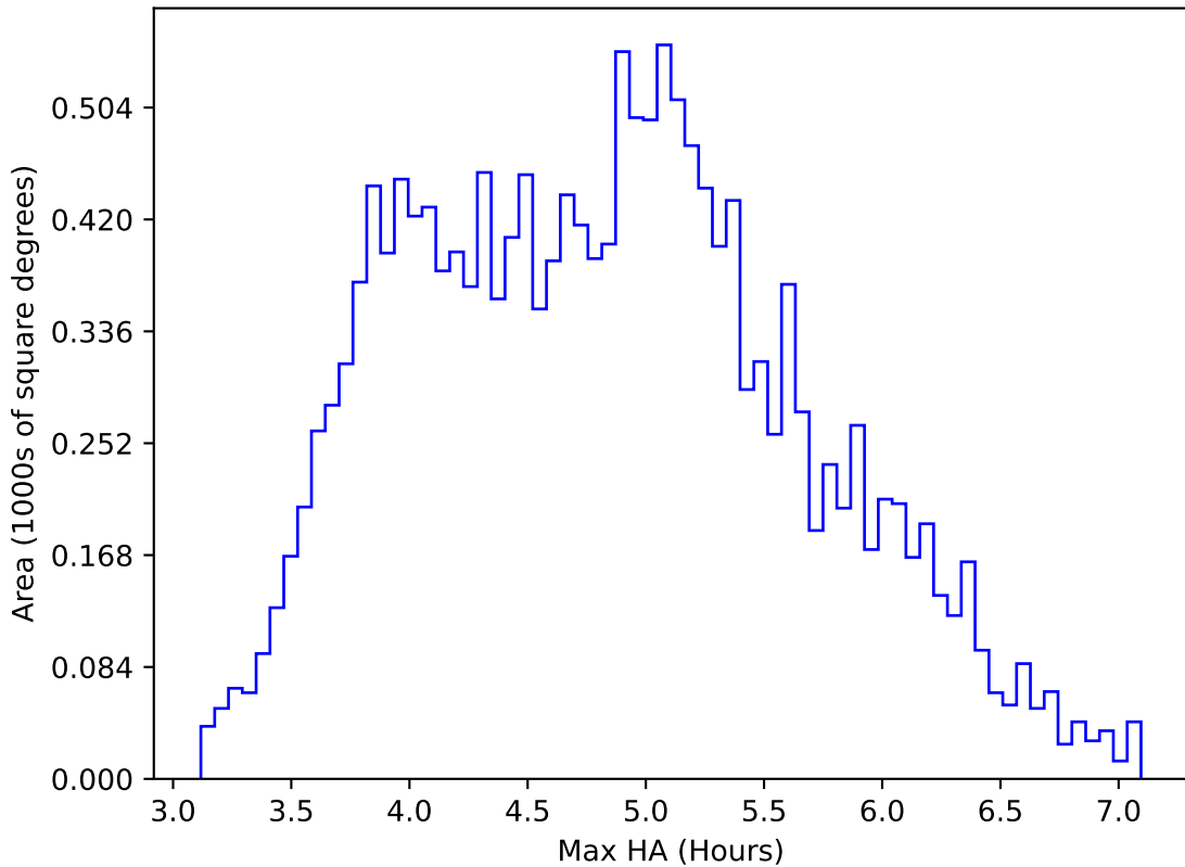
ddf_half_v3.4_10yrs WFD i band: Max HA
