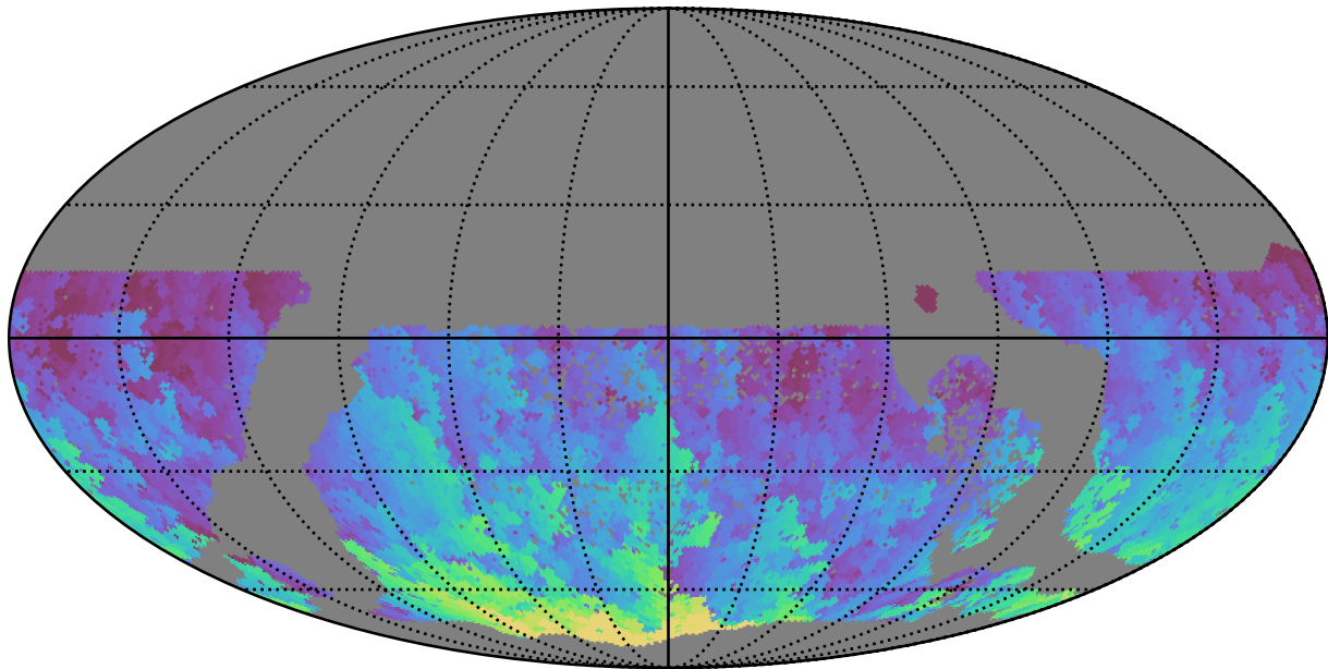
ddf_half_v3.4_10yrs WFD g band: Max HA
