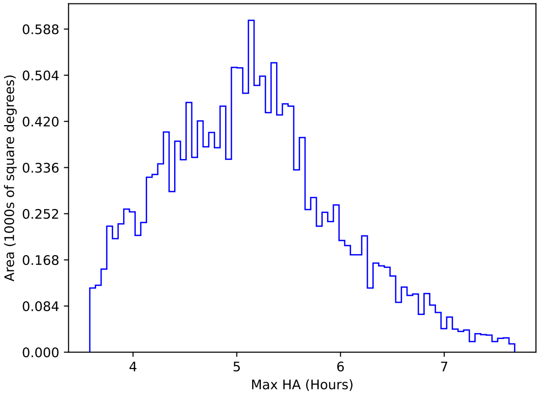
ddf_half_v3.4_10yrs WFD all bands: Max HA
