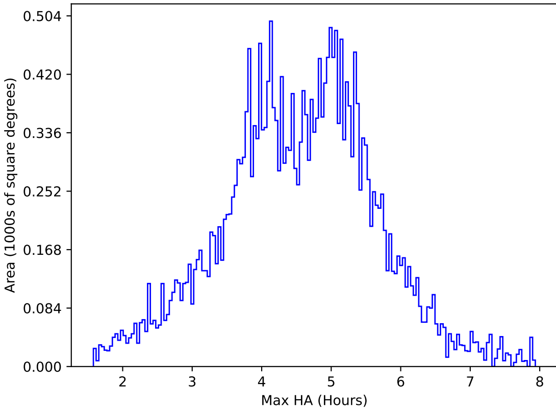
ddf_half_v3.4_10yrs All sky z band: Max HA
