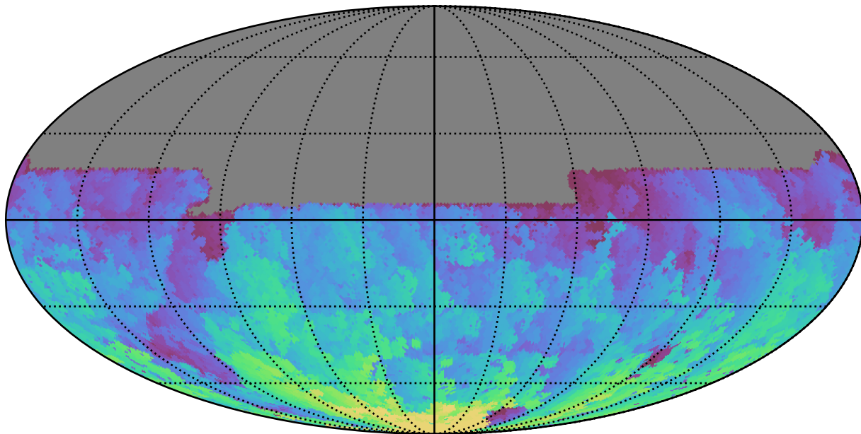
ddf_half_v3.4_10yrs All sky u band: Max HA
