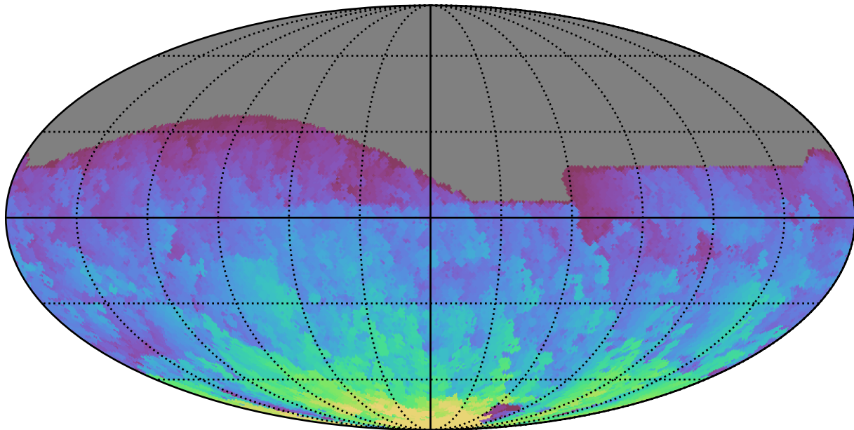
ddf_half_v3.4_10yrs All sky r band: Max HA
