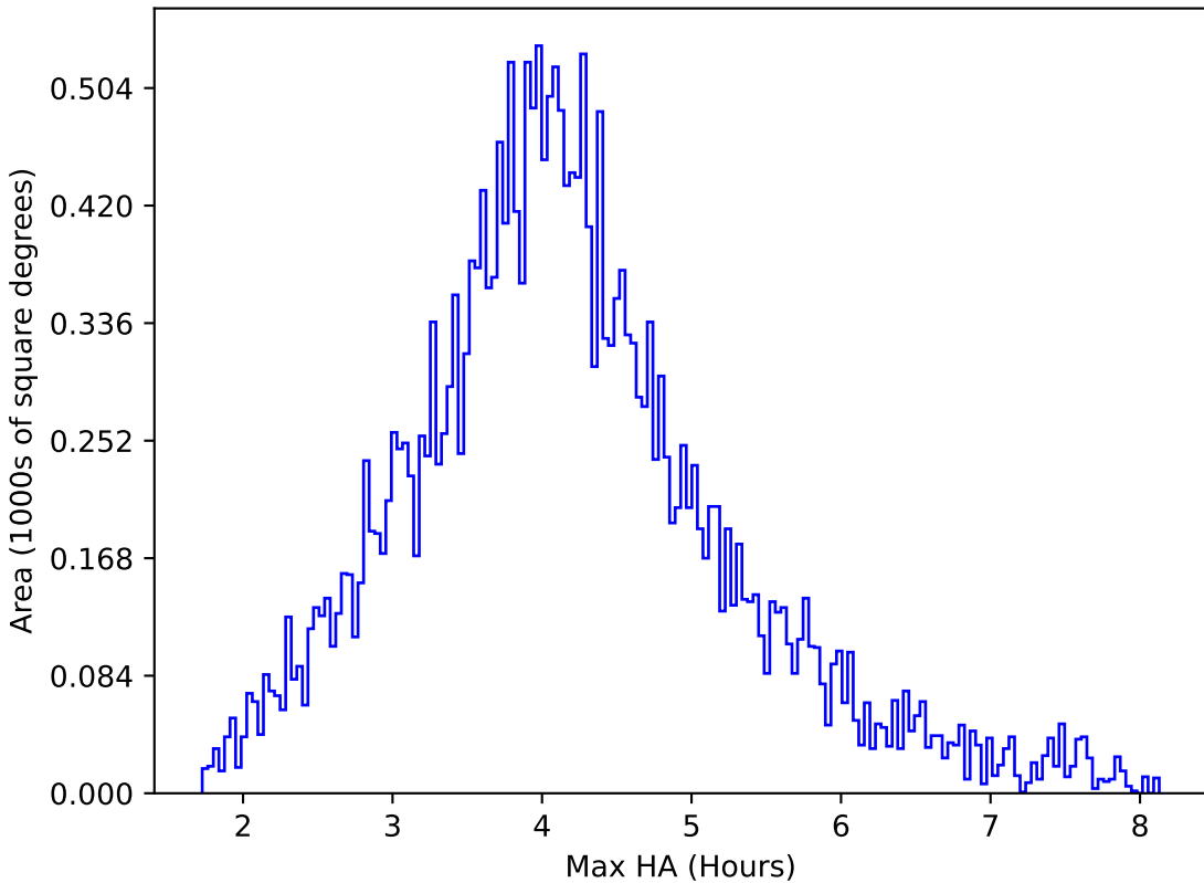
ddf_half_v3.4_10yrs All sky r band: Max HA
