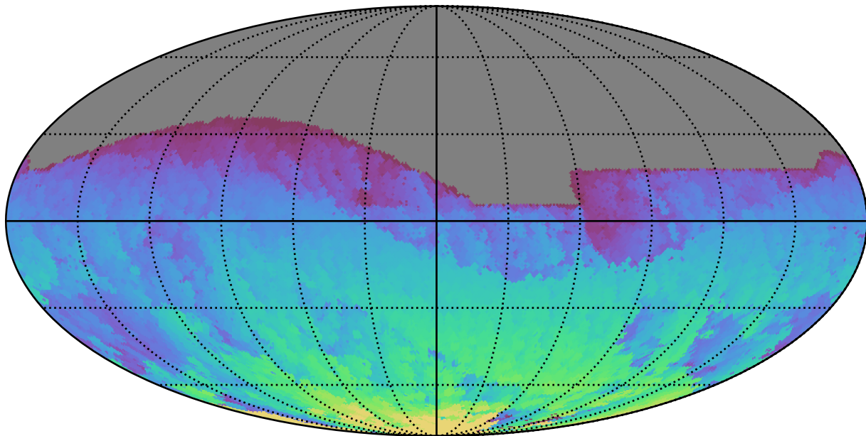
ddf_half_v3.4_10yrs All sky i band: Max HA
