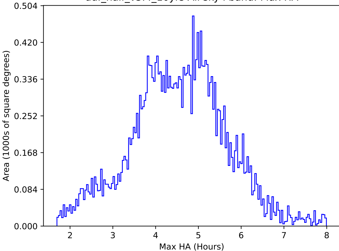
ddf_half_v3.4_10yrs All sky i band: Max HA
