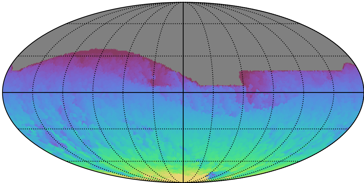
ddf_half_v3.4_10yrs All sky all bands: Max HA
