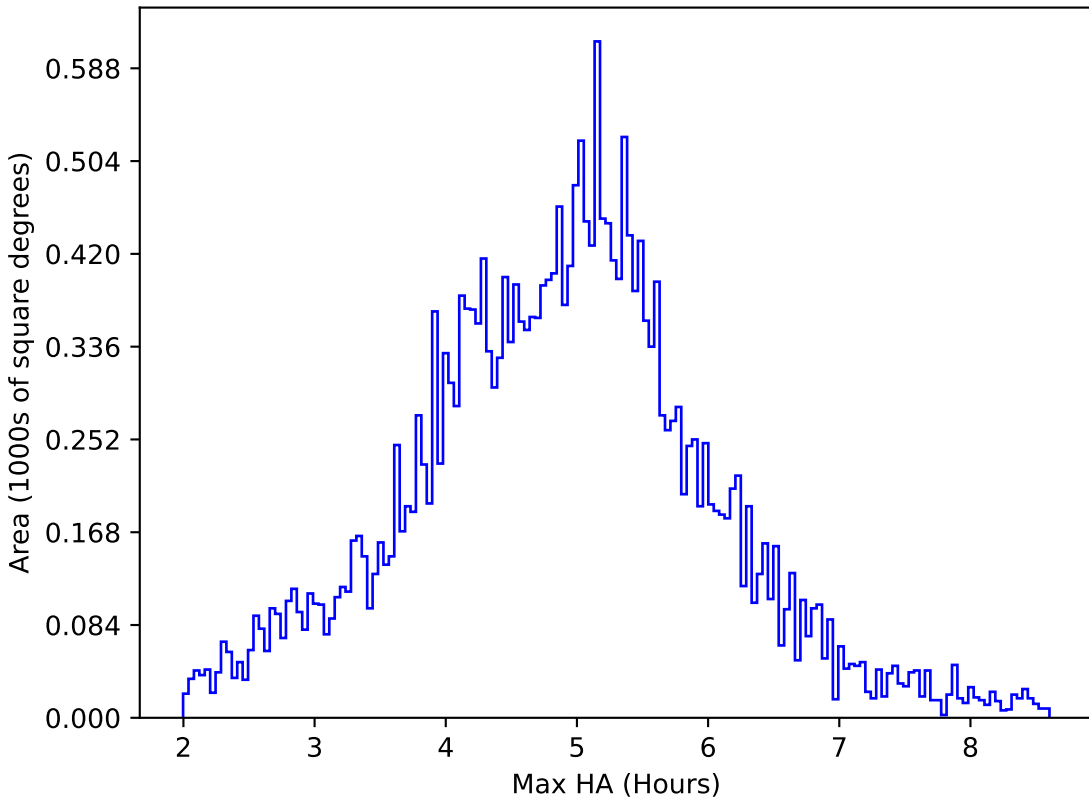
ddf_half_v3.4_10yrs All sky all bands: Max HA
