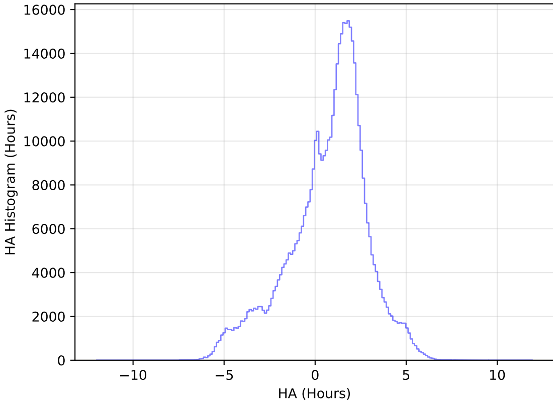
ddf_half_v3.4_10yrs WFD i band: HA Histogram
