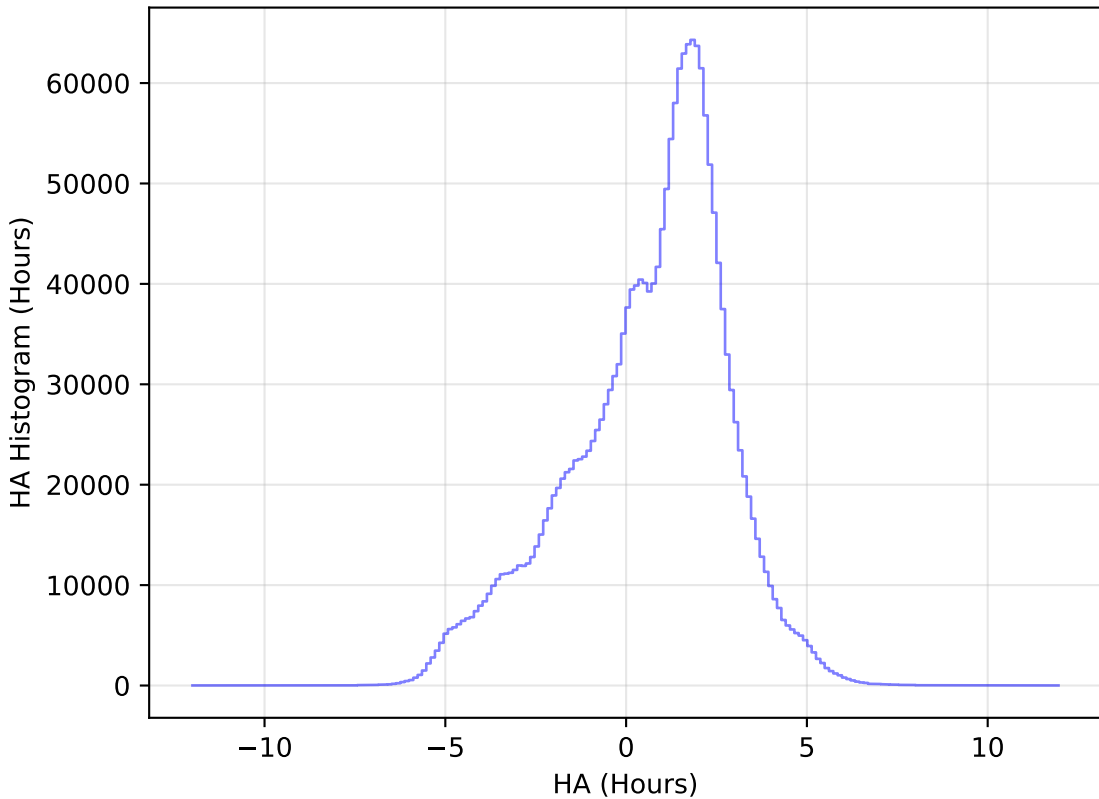
ddf_half_v3.4_10yrs WFD all bands: HA Histogram
