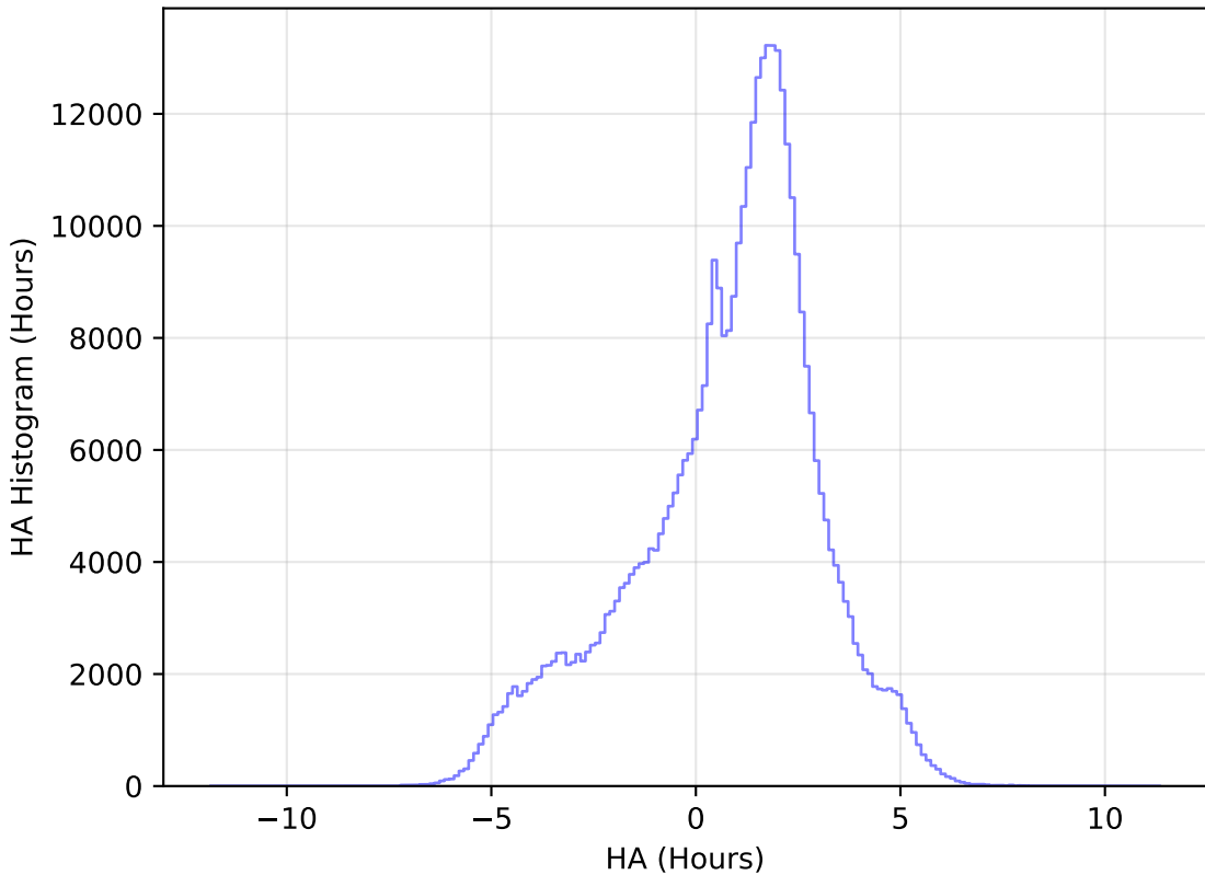
ddf_half_v3.4_10yrs All sky z band: HA Histogram
