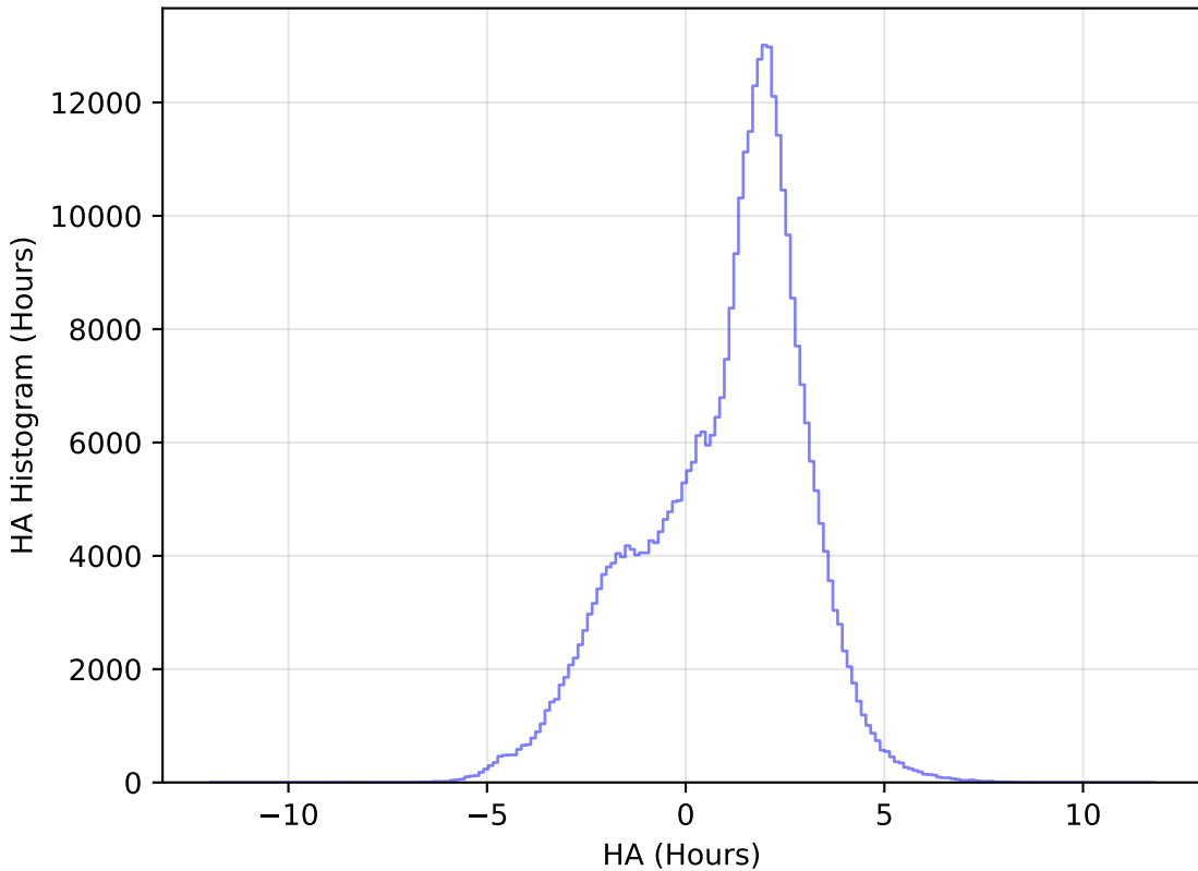
ddf_half_v3.4_10yrs All sky y band: HA Histogram
