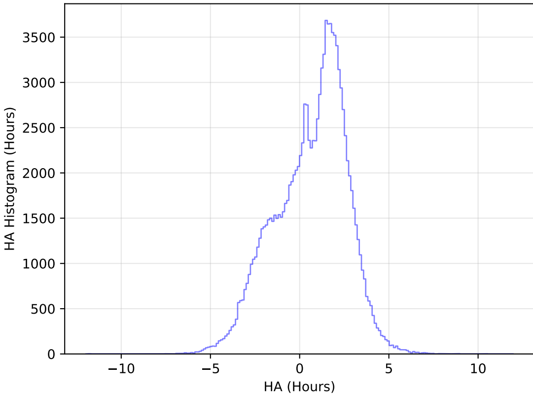
ddf_half_v3.4_10yrs All sky u band: HA Histogram
