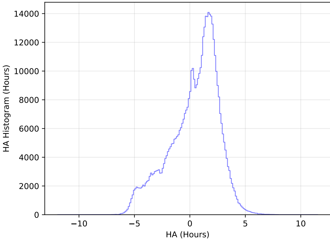
ddf_half_v3.4_10yrs All sky r band: HA Histogram
