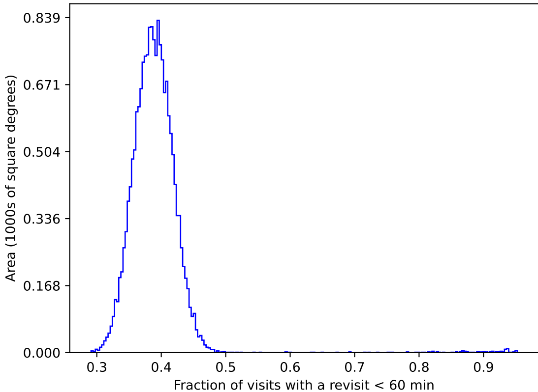
ddf_half_v3.4_10yrs gri WFD: Fraction of visits with a revisit < 60 min
