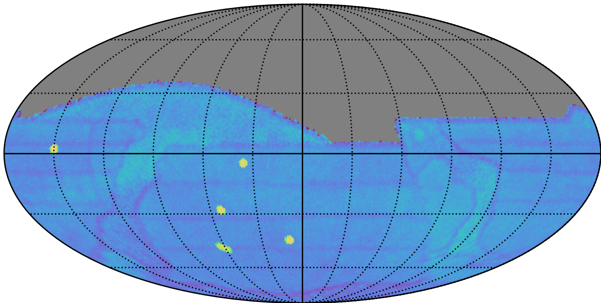
ddf_half_v3.4_10yrs gri All sky: Fraction of visits with a revisit < 60 min
