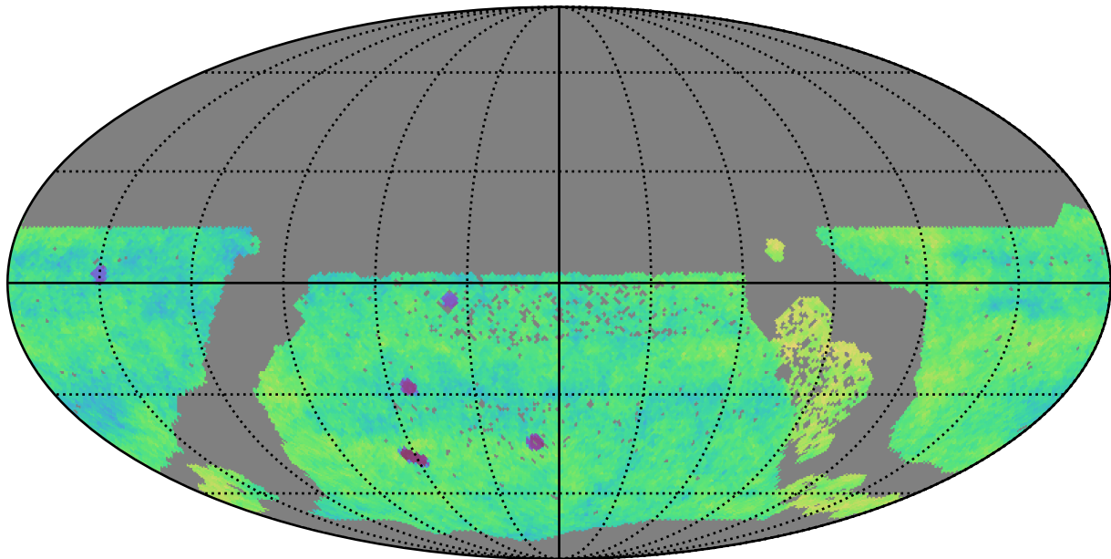
ddf_half_v3.4_10yrs gri WFD: Fraction of visits in pairs (20-90 min)
