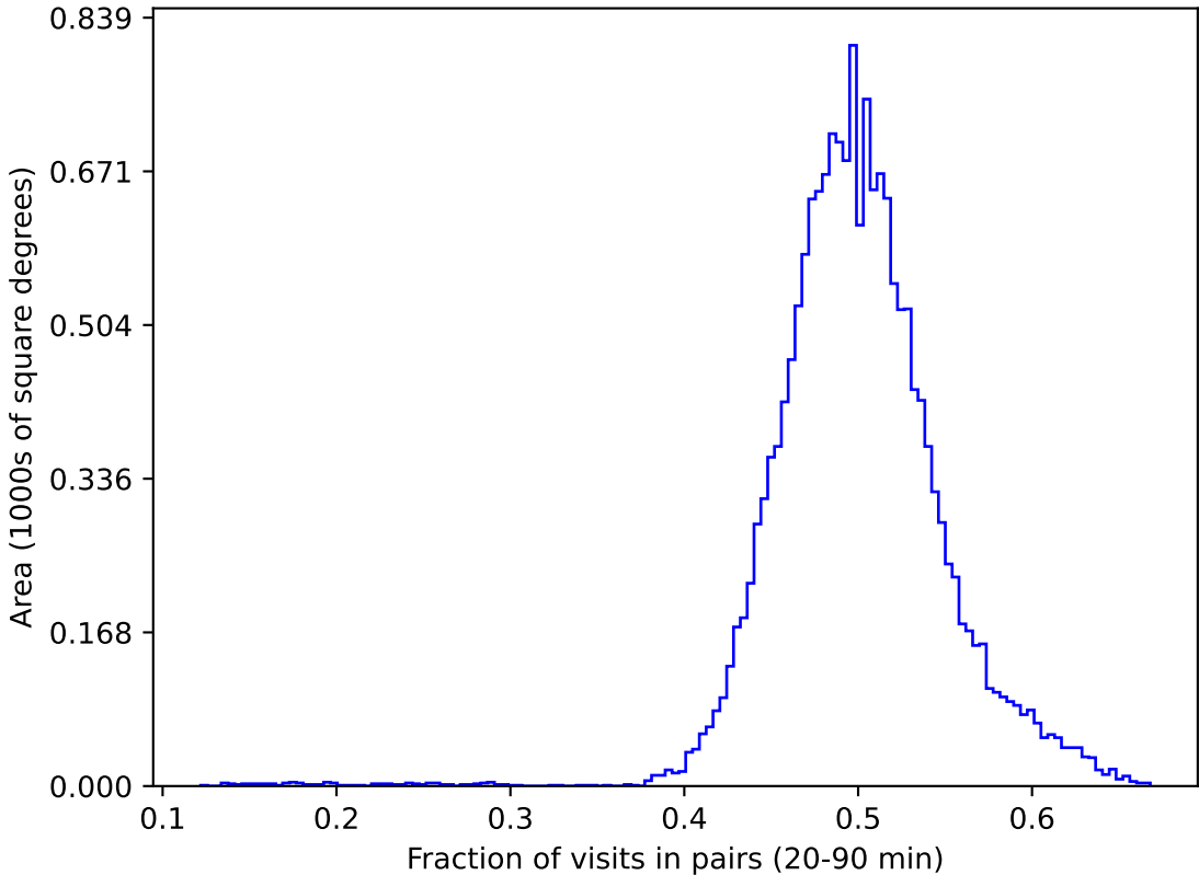
ddf_half_v3.4_10yrs gri WFD: Fraction of visits in pairs (20-90 min)
