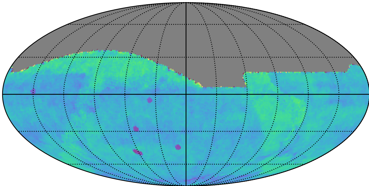
ddf_half_v3.4_10yrs gri All sky: Fraction of visits in pairs (20-90 min)
