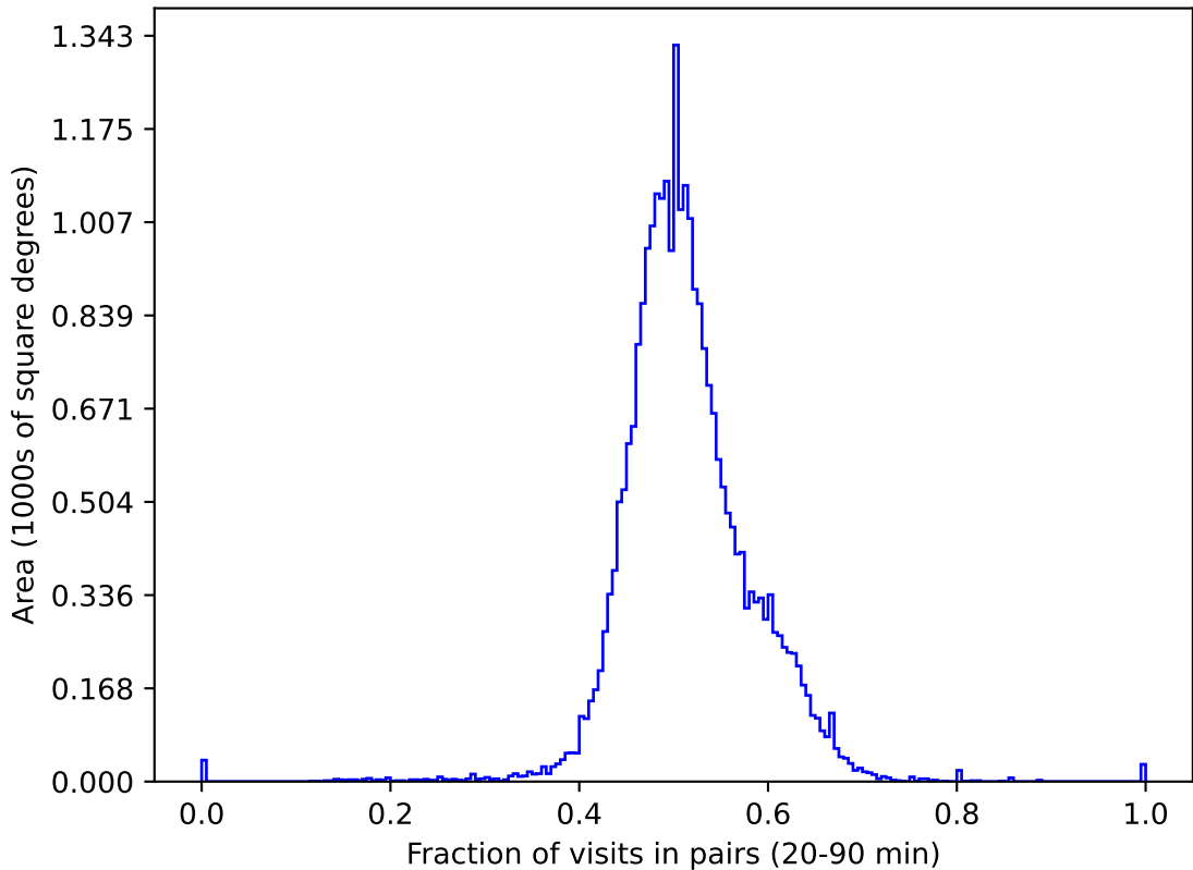
ddf_half_v3.4_10yrs gri All sky: Fraction of visits in pairs (20-90 min)
